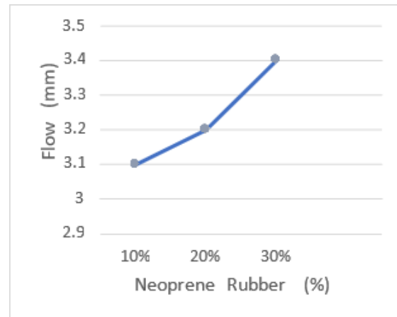
Rajah 5. Flow
