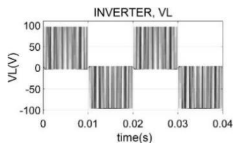
Rajah 17: Voltan Penyongsang
