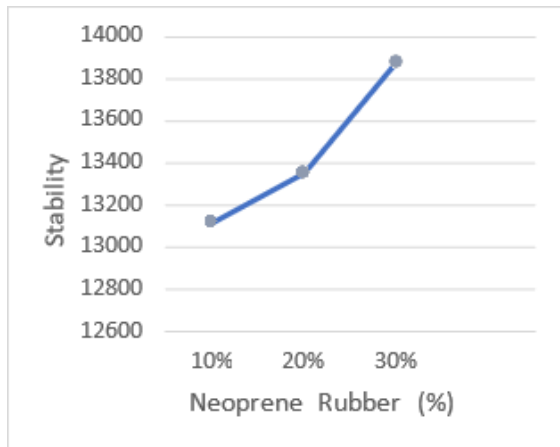
Rajah 4. Stability
