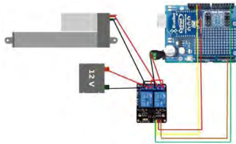
Figure 5. Circuit of Smart Pedal Lock
