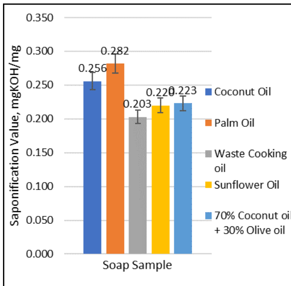
Figure 10. Saponification value
