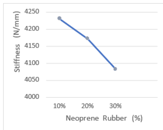
Rajah 6. Stiffness
