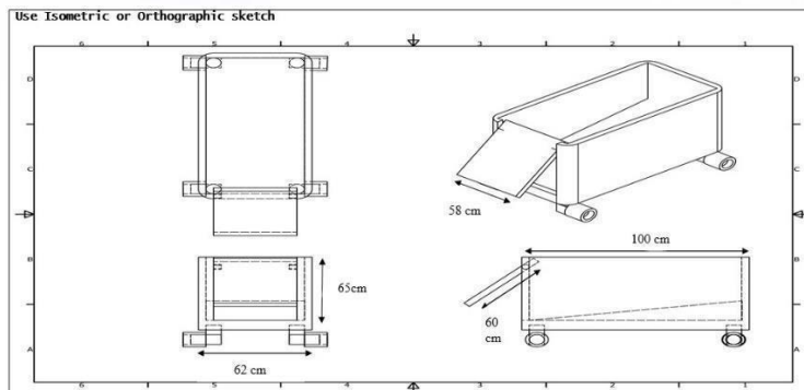
Rajah 4.1 Lakaran lukisan isometrik Scrap Rubber Carrier
