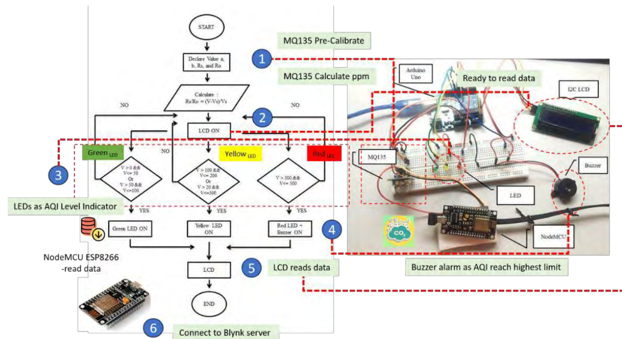
Figure 4. Flowchart of Air Quality Monitoring System (AQMs) and hardware setup
