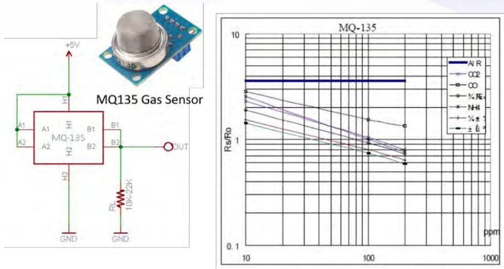
Figure 2. Gas concentration graph of the MQ135 gas sensor
